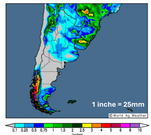
GFS High-Resolution Precipitation Forecast Days 1-7: 00UTC 6 Feb 2025 - 00UTC 13 Feb 2025 Model Initialized 00UTC 5 Feb 2025
